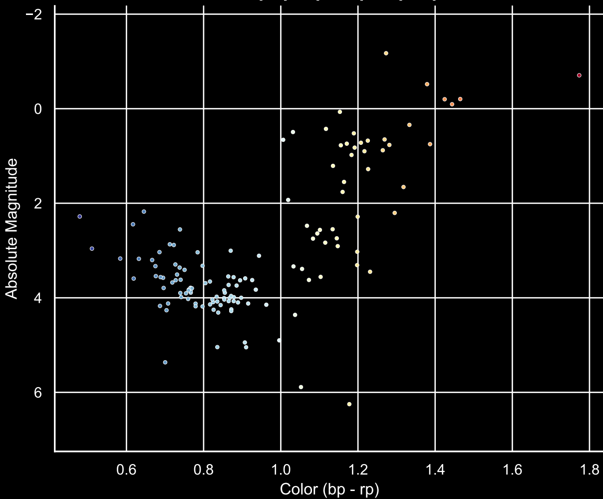
GALAH Hertzprung-Russel Diagram Field [114] Ra [327.63] Dec [-6.55]
