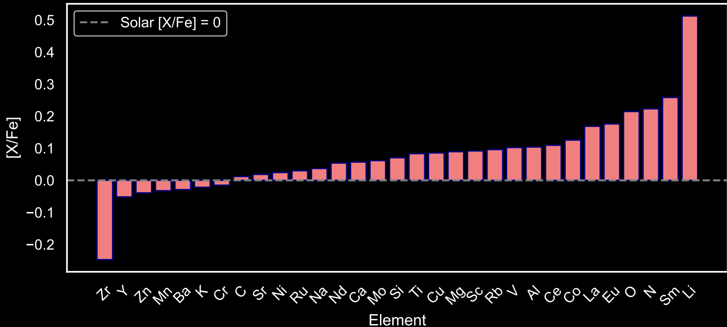
Abundance Pattern for GALAH Star Field [114] (N=132)
