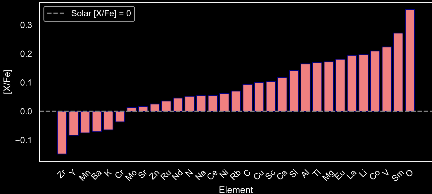
Abundance Pattern for GALAH Red Giants: Star Field [114] (N=41)
