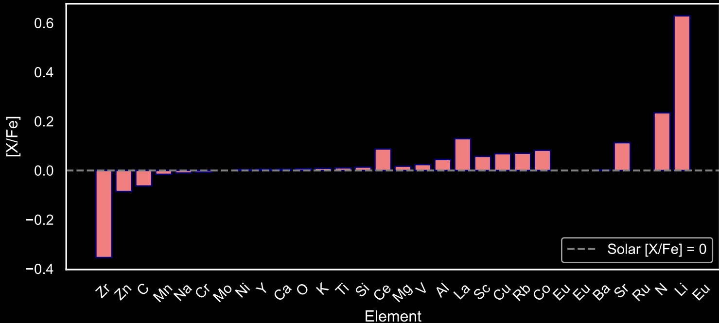
Abundance Pattern for GALAH Main Sequence Stars: Star Field [114] (N=23)
