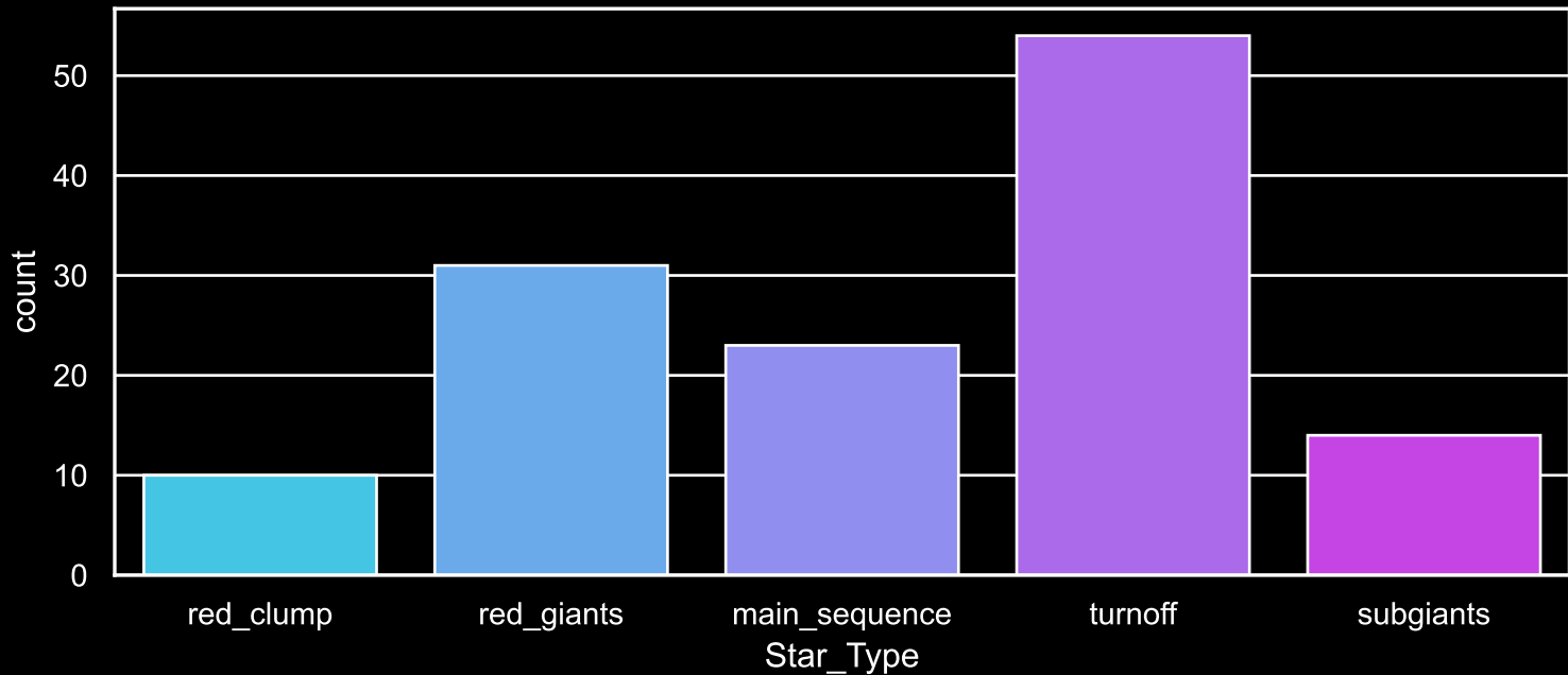
Field [114] Count plot of Star Type
